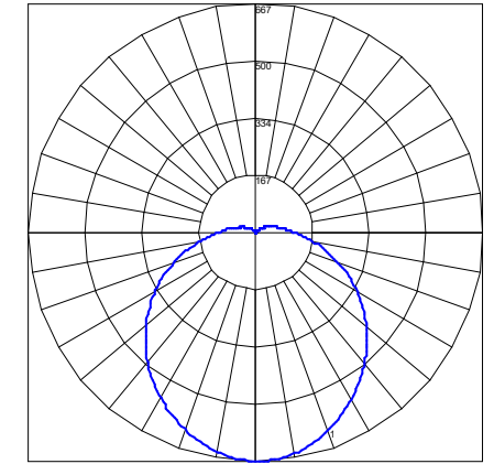
Maximum Candela = 667.283 Located At Horizontal Angle = 0, Vertical Angle = 0 # 1 - Vertical Plane Through Horizontal Angles (0 - 180) (Through Max. Cd.)
