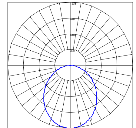
Maximum Candela = 1235.166 Located At Horizontal Angle = 90, Vertical Angle = 1 # 1 - Vertical Plane Through Horizontal Angles (90 - 270) (Through Max. Cd.)
